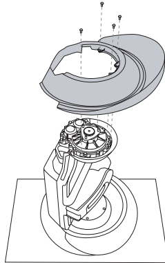
Figure 40. Servicing the Fenders
